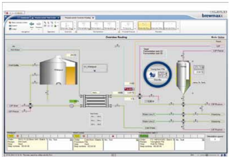
Fig. 3: Visualisation of process flow on a process control system
